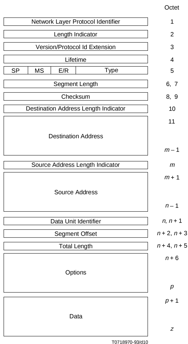
Figure 9 – Data PDU
