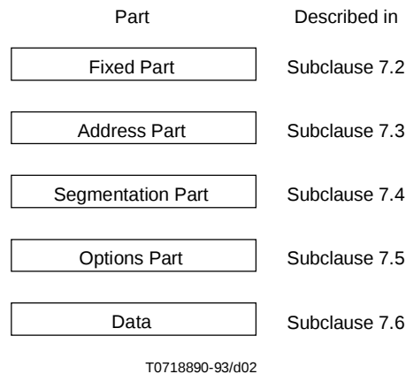
Figure 1 – PDU structure
