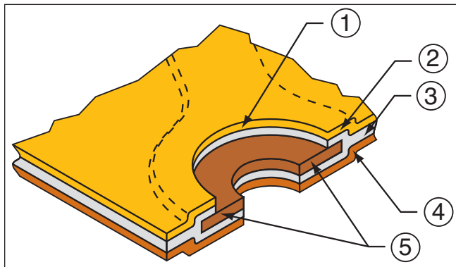
Figure 1-1 Type 1 Single-sided Flexible Printed Board - Adhesive Substrate Construction
